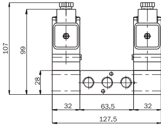
Dik Bobinli Valf Vertical type solenoid SV-1/4-5/2-B-B
